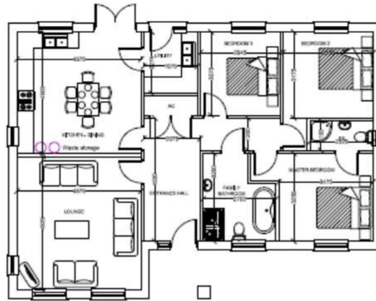
Proposed Ground Floor Plan 1105
